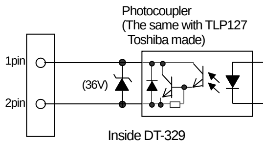
[Output circuit]
