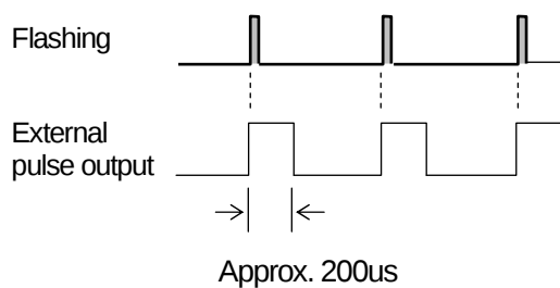
[Output time]
