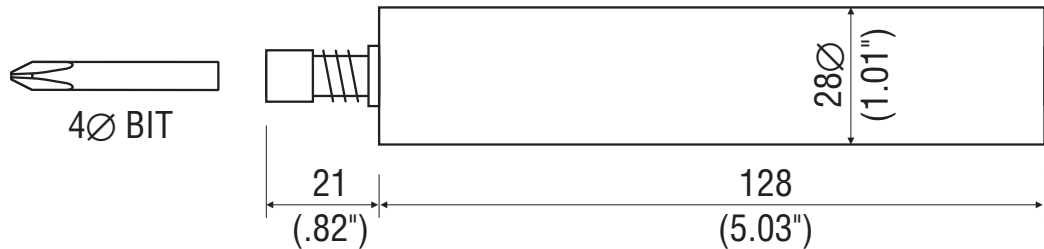
NTS-6-S3 DETECTOR 37 \varnothing (1.45") x 195 (7.67")
