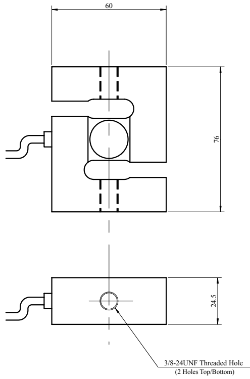
DPU-220 Dimensions in mm
