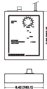
CONTROL UNIT
